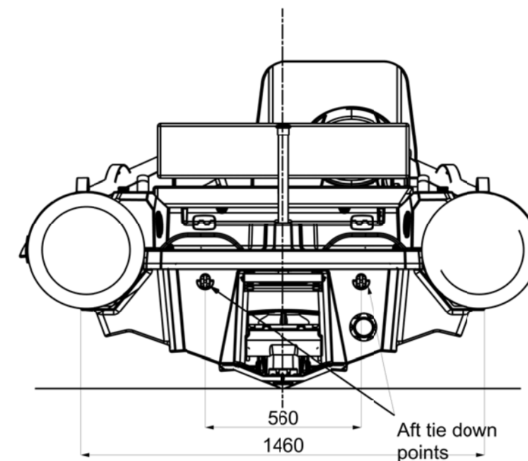
AFT VIEW
