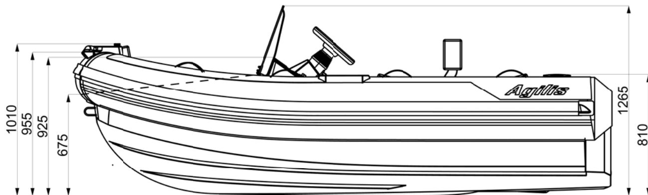
SIDE VIEW
