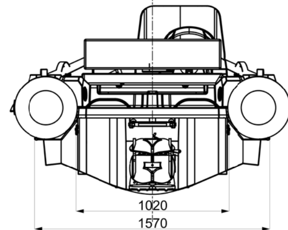
AFT VIEW
