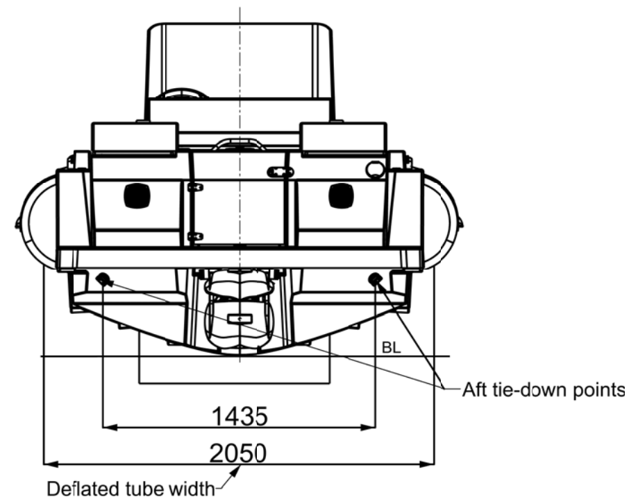
AFT VIEW
