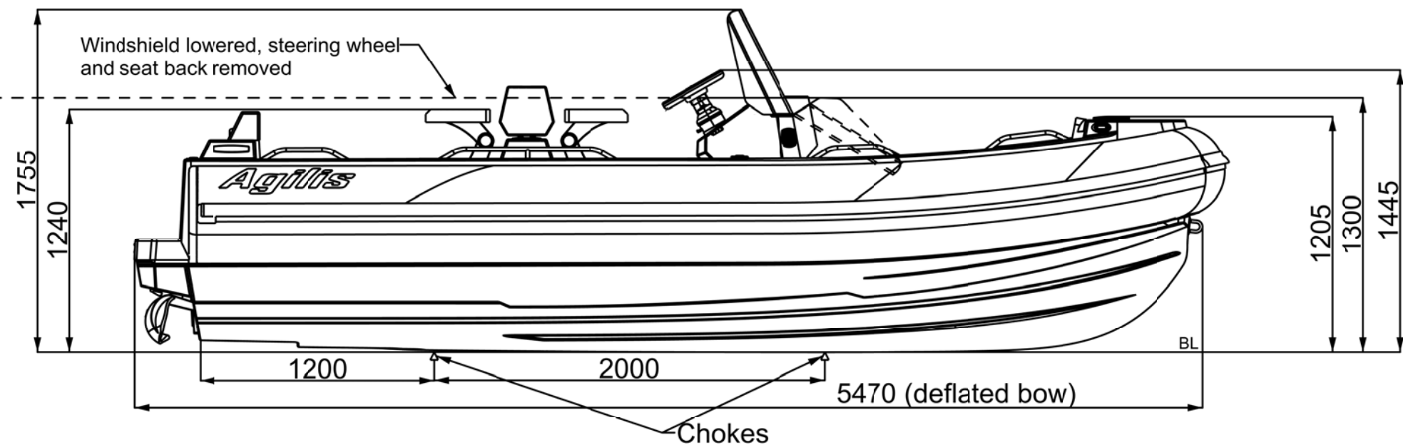
SIDE VIEW (reduced profile with single lifting point, optional)
