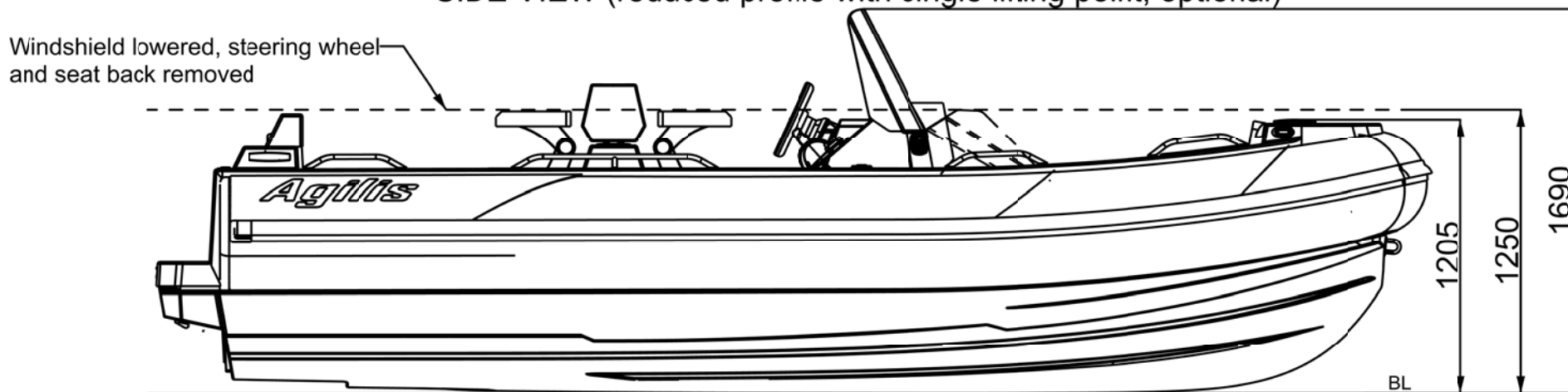
SIDE VIEW (reduced profile with single lifting point, optional)
