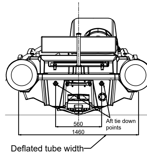
AFT VIEW
