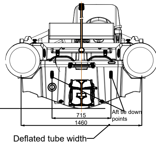
AFT VIEW
